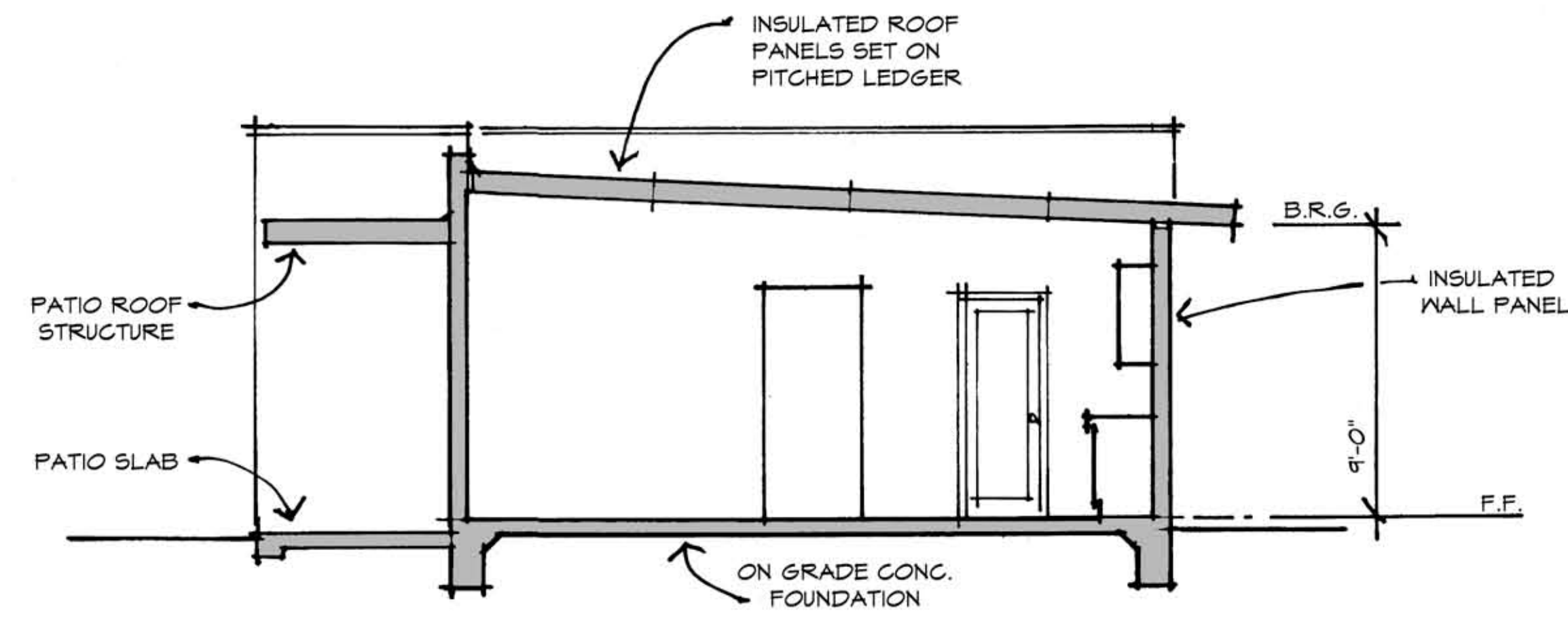
SECTION
