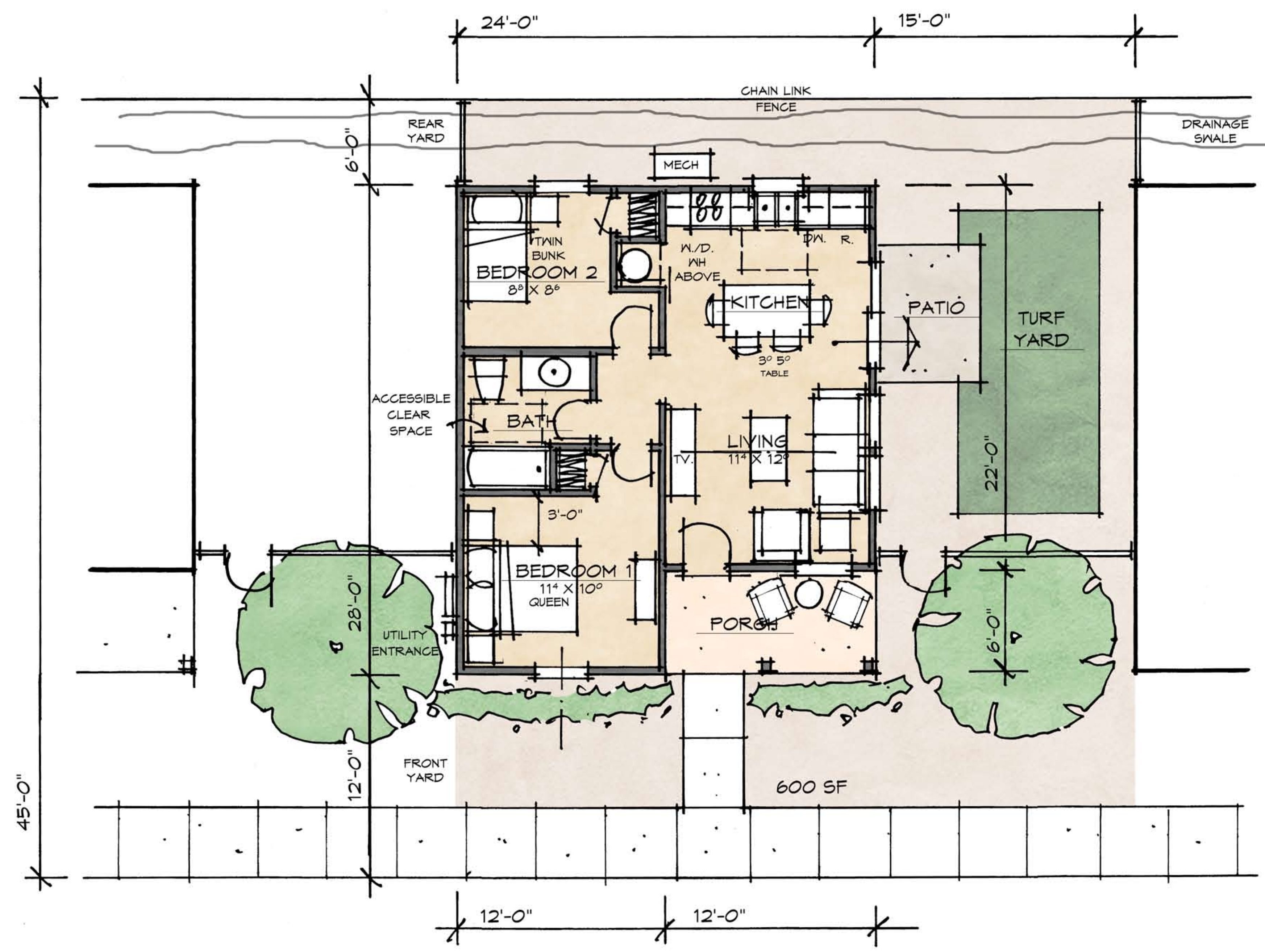
FLOOR PLAN 600 SF
