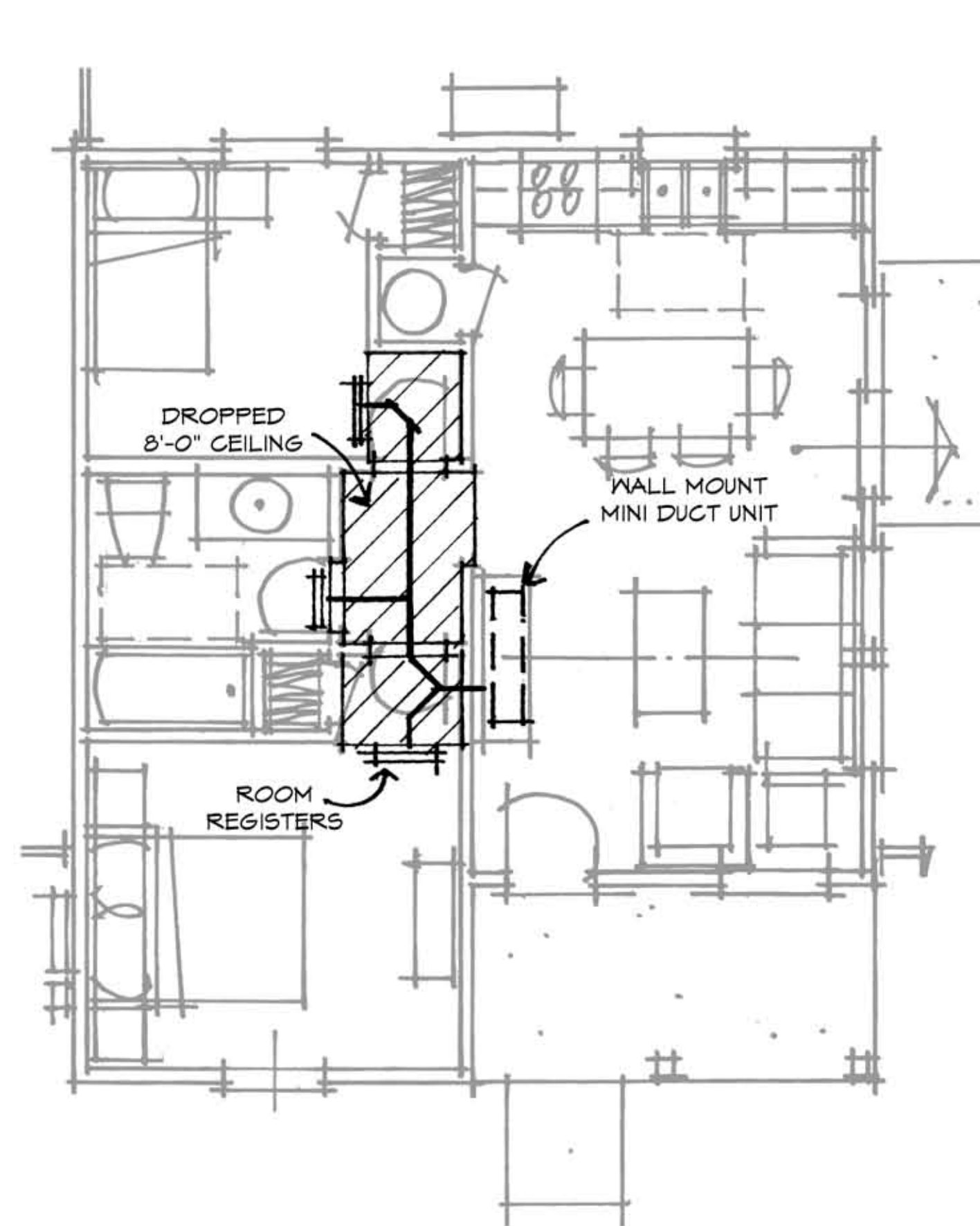
MECHANICAL PLAN
