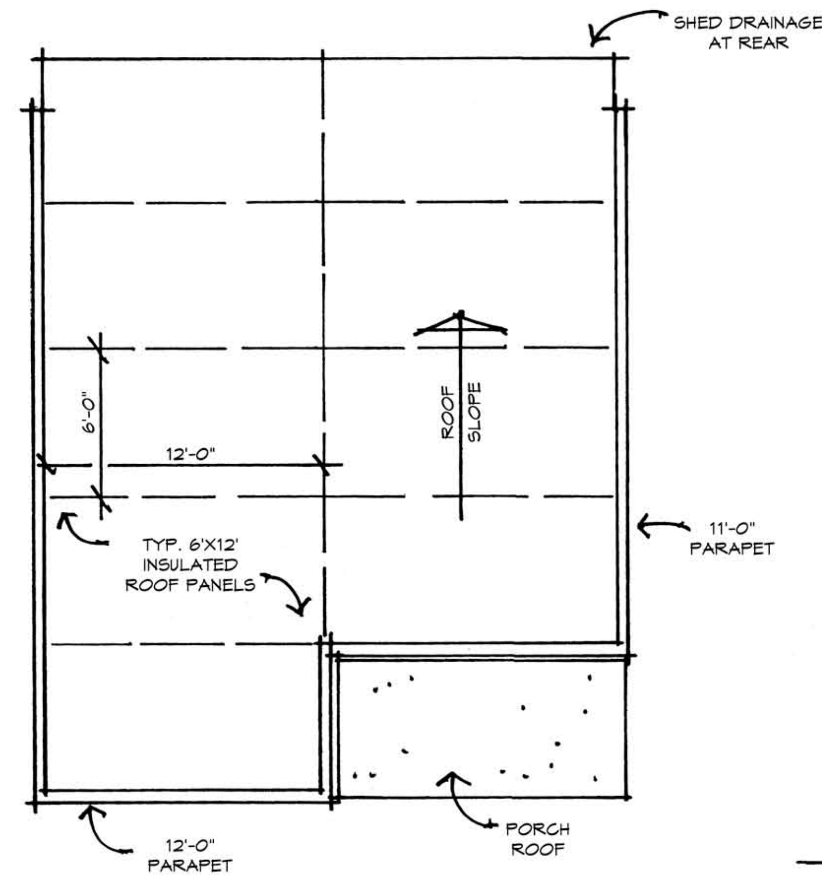
ROOF PLAN
