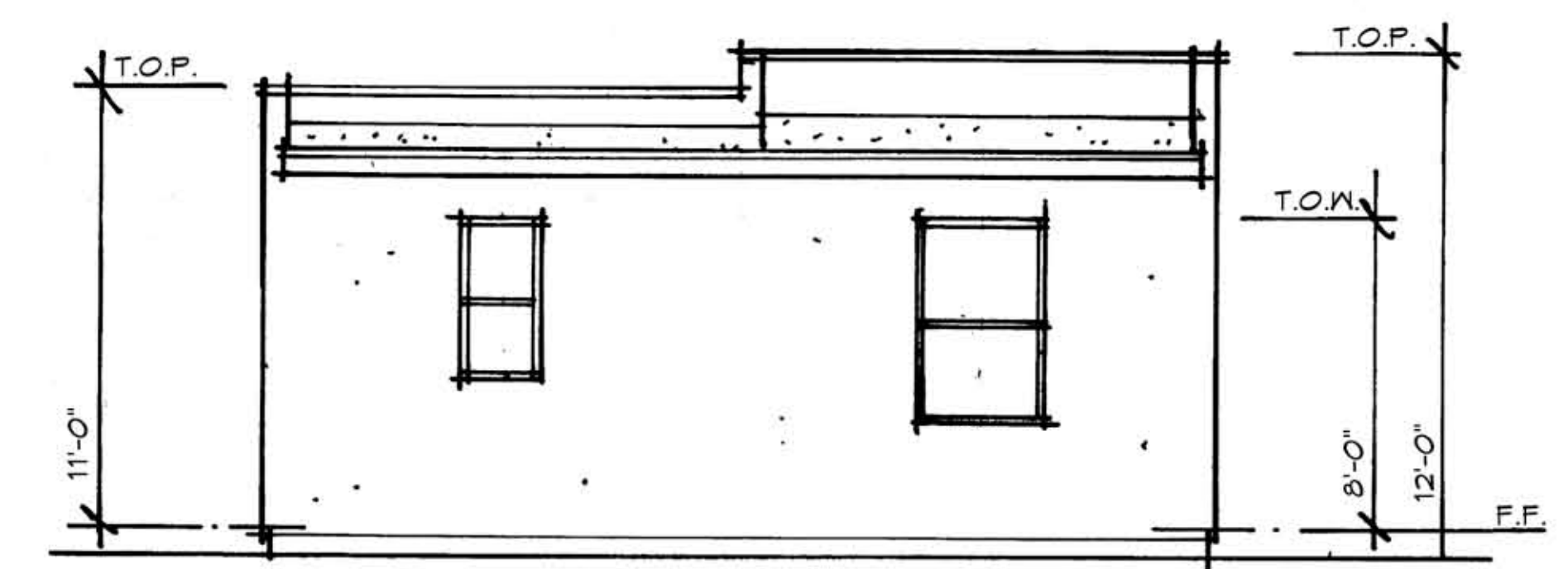
REAR ELEVATION
